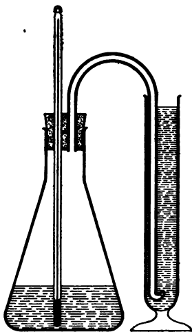
FIG. 27. — Apparatus for the demonstration of the release of carbon dioxide in fermentation; \times \frac{1}{2} .
